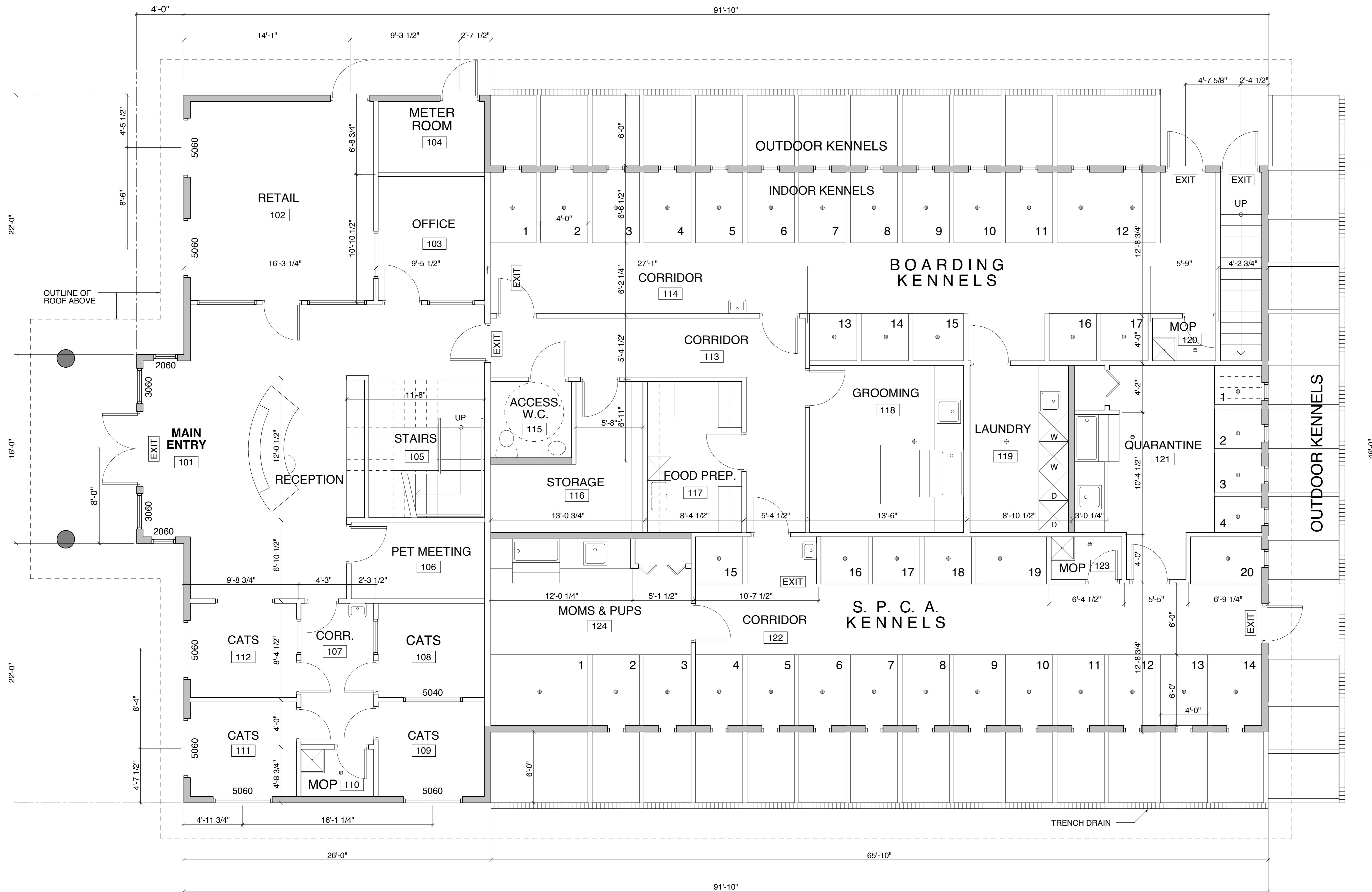
1 GROUND FLOOR A2-02 SCALE: 1/4" = 1'-0"
